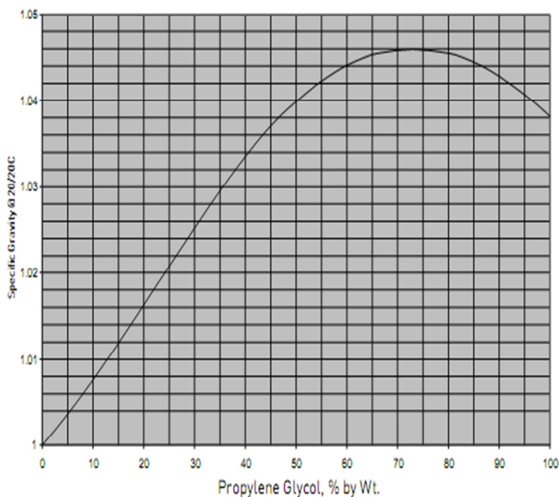
Specific Gravity of Aqueous Propylene Glycol Solutions
